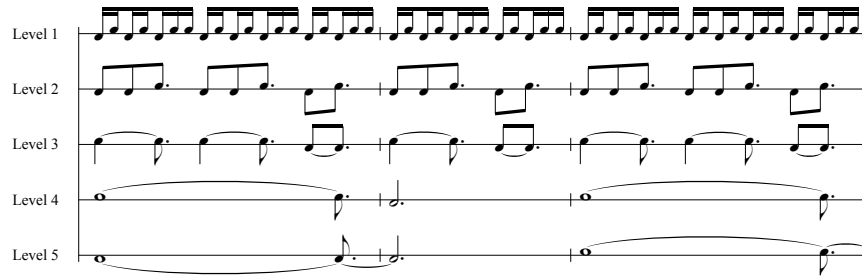
Fig. 3. Realization of c_{\sqrt{10}/2}
